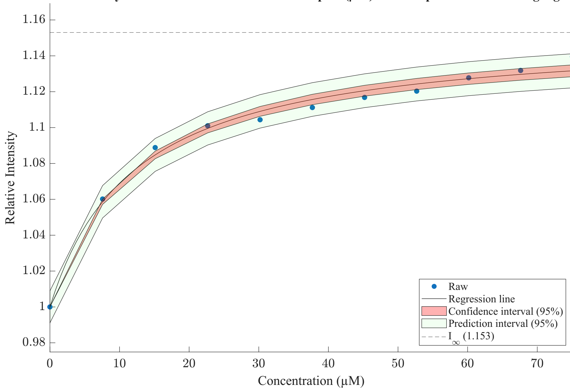
Relative intensity as a function of concentration of lipids ( \mu\text{M} ) for wt rep3 - Statistics fitting algorithm
